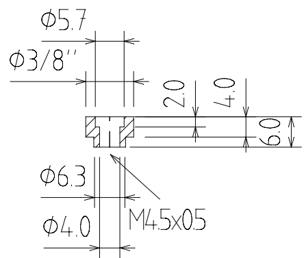
Gas filler valve bushing (#114)
